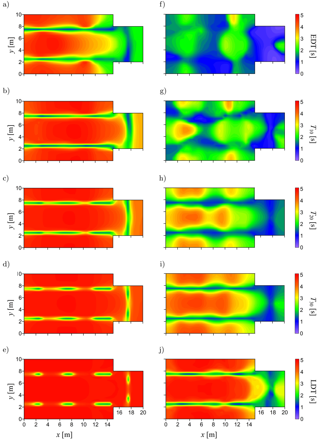
FIG. 13. Distribution of decay times EDT, T_{10} , T_{20} , T_{30} , LDT on observation plane for octave band 31.5 Hz and source located in: a)–e) subroom A and f)–j) subroom B.
