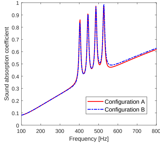
FIG. 11. Sound absorption coefficient.
