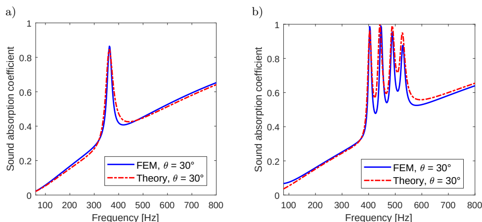
FIG. 9. Sound absorption coefficient for oblique incidence: a) one embedded resonator, b) four embedded resonators.
