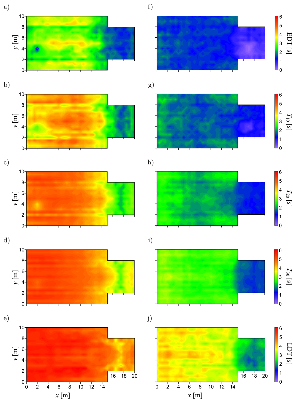
FIG. 10. Distribution of decay times EDT, T_{10} , T_{20} , T_{30} , and LDT on observation plane for source located in: a)–e) subroom A and f)–j) subroom B.
