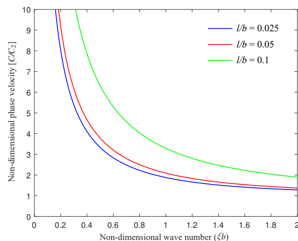
FIG. 6. Phase velocity profiles for illustrating impact of dimensionless parameter ( l/b ) on symmetric SH-waves.
