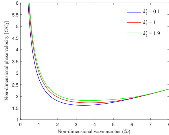
FIG. 7. Phase velocity profiles for illustrating impact of dimensionless shear stiffness parameter ( k_1^* ) on symmetric SH-waves.
