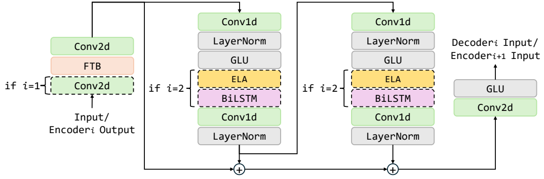
FIG. 2. Structure of encoder.
