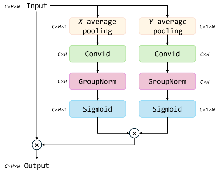
FIG. 3. Efficient local attention.
