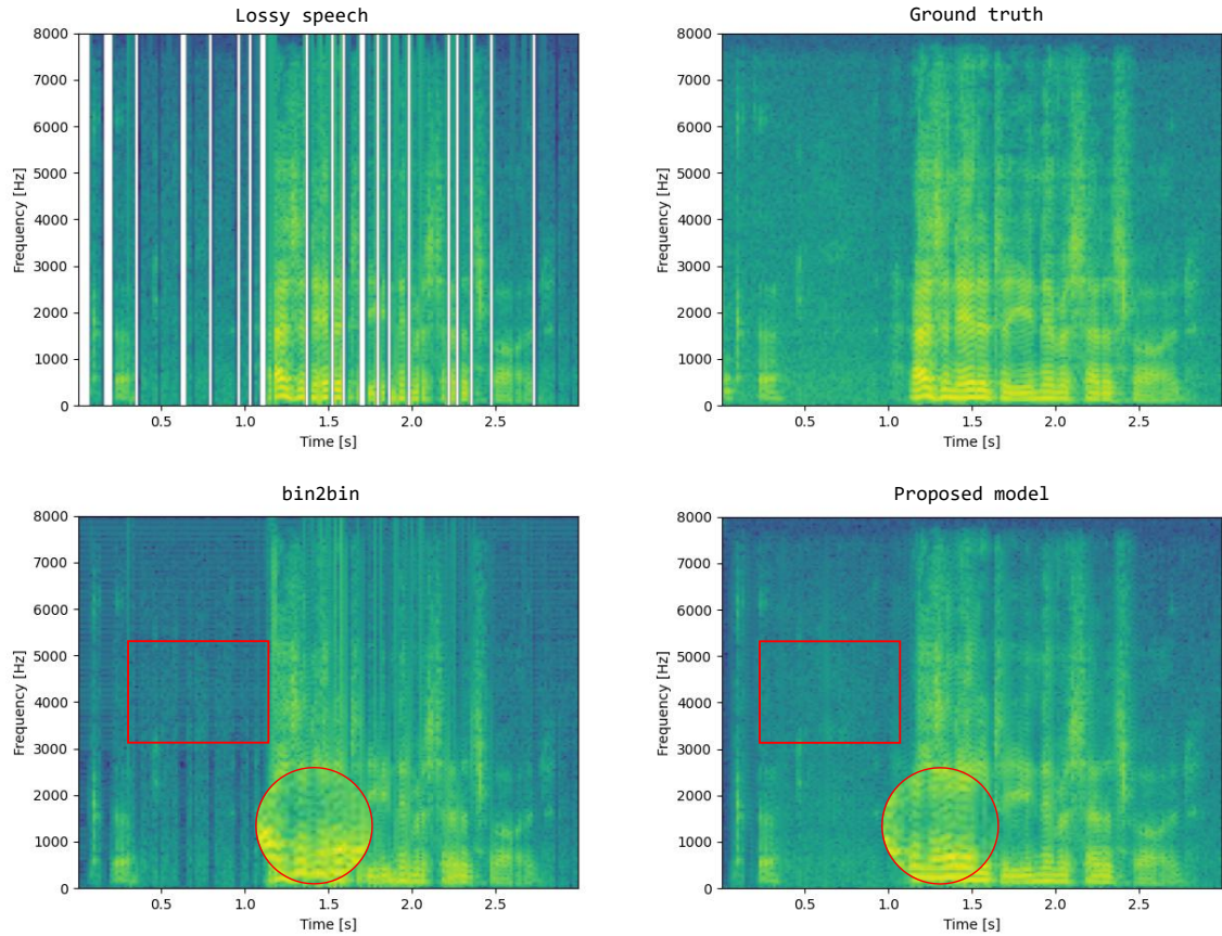
FIG. 7. Visualization of the output spectrogram.
