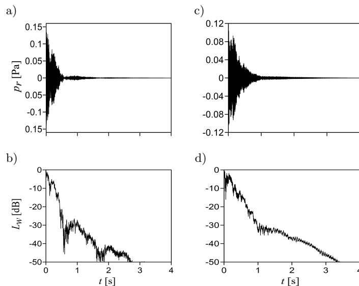
FIG. 7. Variations in the sound pressure p_r and the pressure level L_w at receiving point for excitation frequency: a), b) 104 Hz, c), d) 257 Hz. Sound source located in subroom B.
