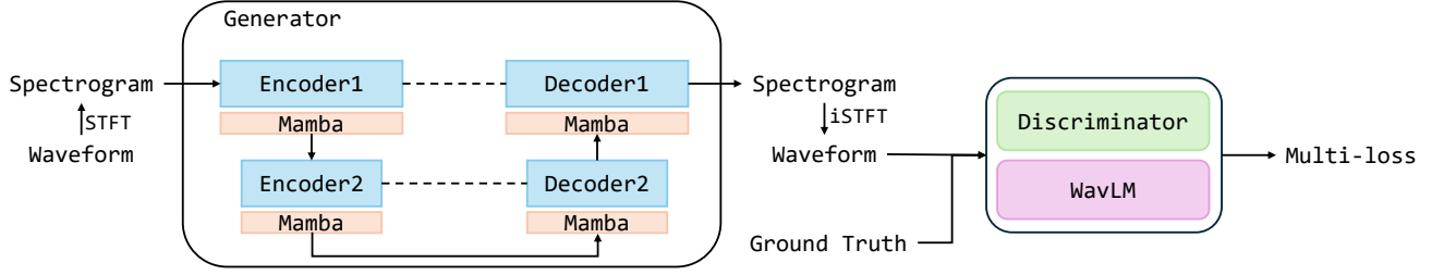
FIG. 1. Structure of proposed generative adversarial network.
