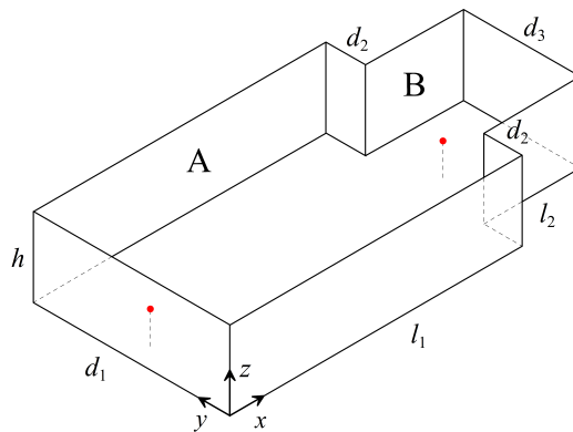
FIG. 2. Room system under investigation containing two connected rectangular rooms marked with letters A and B. Red dots indicate locations of the sound source.
