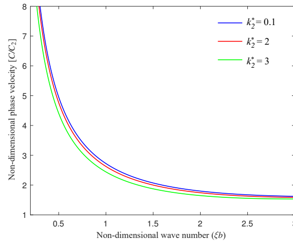
FIG. 8. Phase velocity profiles for illustrating impact of dimensionless rotational stiffness parameter ( k_2^* ) on symmetric SH-waves.
