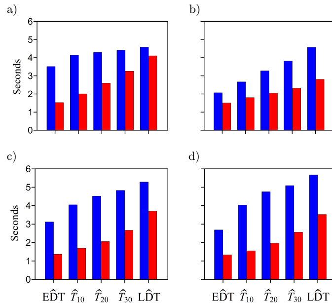
FIG. 12. Mean decay times EDT, \hat{T}_{10} , \hat{T}_{20} , \hat{T}_{30} , LDT on observation plane in subroom A for octave bands: a) 31.5 Hz, b) 63 Hz, c) 125 Hz, d) 250 Hz. Results marked with blue and red bars correspond to source located in subrooms A and B, respectively.
