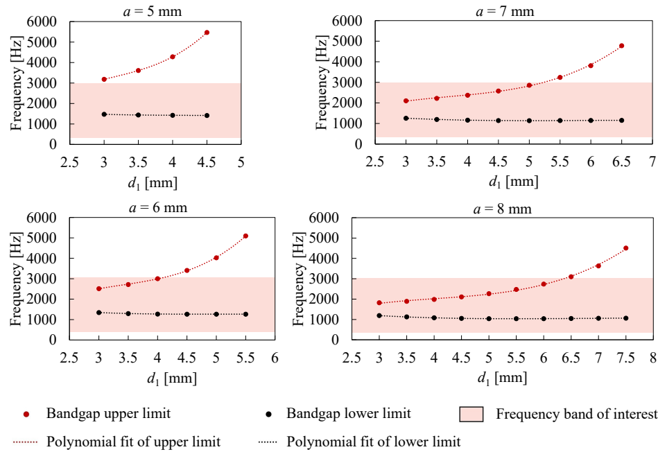
FIG. 8. Bandgap characteristics of metamaterial model 2 with 0.2 mm thick rubber layer for varying diameters of inclusion in unit cell with lattice constants, depicting the overlap of the bandgaps with the frequency range of interest.
