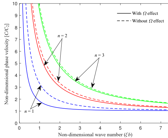
FIG. 1. Phase velocity profiles for illustrating modes of symmetric SH-waves.
