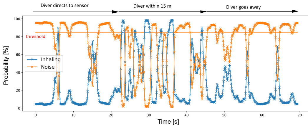
FIG. 12. Model prediction for diver signal 'Diver_3.'
