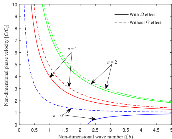
FIG. 2. Phase velocity profiles for illustrating modes of anti-symmetric SH-waves.
