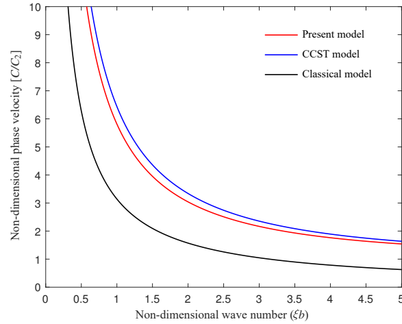
FIG. 11. Phase velocity profiles for illustrating symmetric SH-waves behavior under different models.
