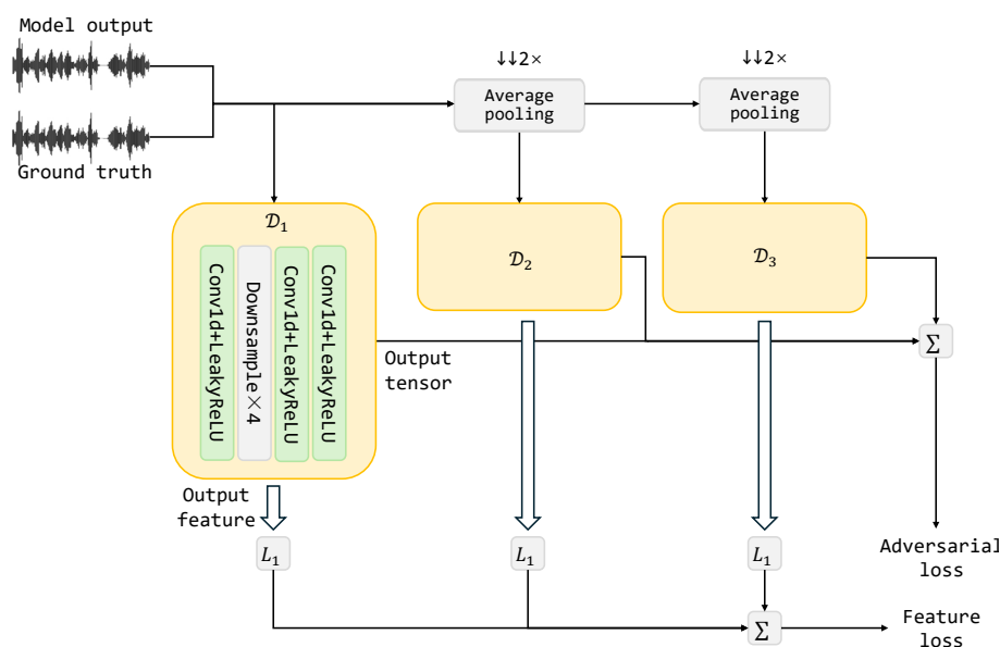
FIG. 5. Structure of discriminator.
