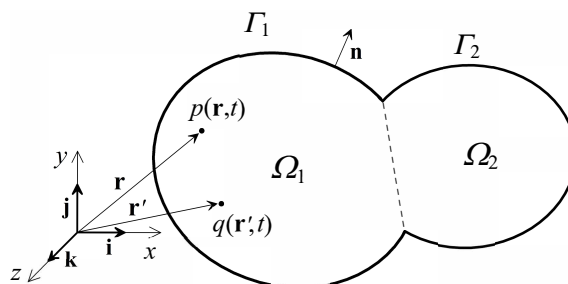
FIG. 1. Analyzed system consisting of two enclosed spaces \Omega_1 and \Omega_2 connected by a transparent opening denoted by dashed line.
