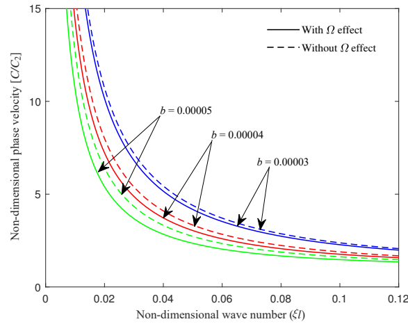
FIG. 4. Phase velocity profiles for illustrating impact of varying plate thickness on symmetric SH-waves.
