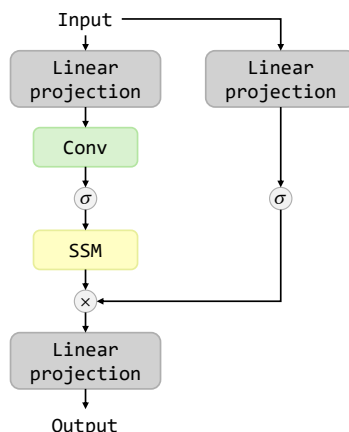
FIG. 4. Mamba block.
