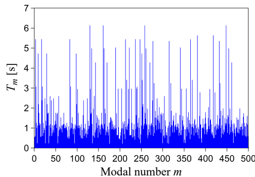
FIG. 9. Modal reverberation time T_m for first 500 eigenmodes.
