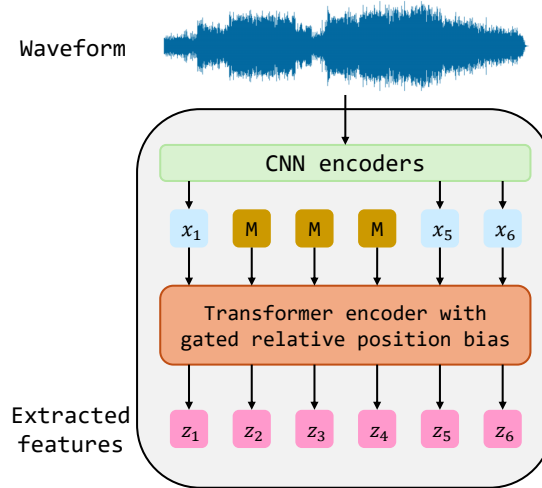
FIG. 6. Structure of WavLM.
