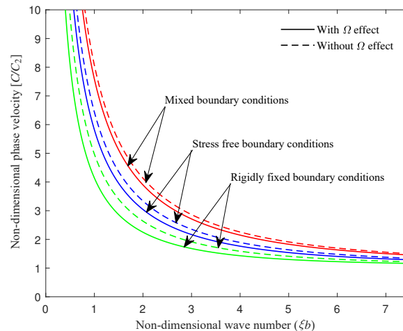
FIG. 9. Phase velocity profiles for illustrating impact of boundary conditions on symmetric SH-waves.
