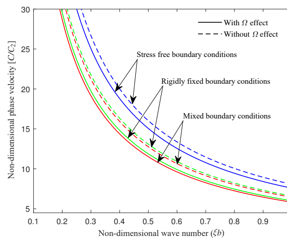
FIG. 10. Phase velocity profiles for illustrating impact of boundary conditions on anti-symmetric SH-waves.
