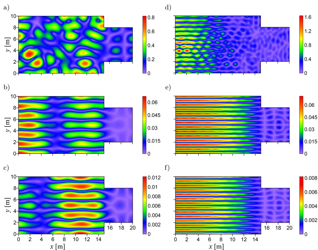
FIG. 4. Changes in the pressure amplitude P (in pascals) on observation plane for excitation frequency: a)–c) 104 Hz, d)–f) 257 Hz, and the time t : a), d) 0 s, b), e) 2 s, c), f) 4 s. Sound source located in subroom A.
