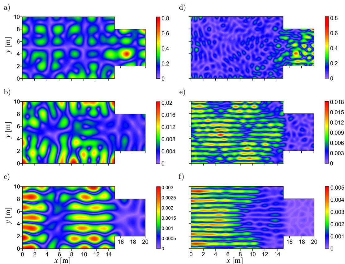
FIG. 6. Changes in the pressure amplitude P (in pascals) on observation plane for excitation frequency: a)–c) 104 Hz, d)–f) 257 Hz, and the time t : a), d) 0 s, b), e) 1 s, c), f) 2 s. Sound source located in subroom B.
