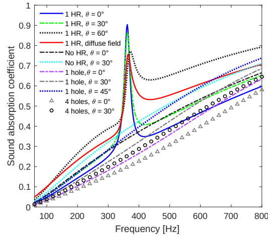
FIG. 12. Sound absorption coefficient of the metamaterial.
