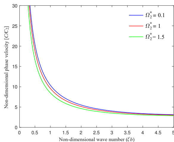
FIG. 3. Phase velocity profiles for illustrating impact of dimensionless rotation parameter \Omega_2^* on symmetric SH-waves.
