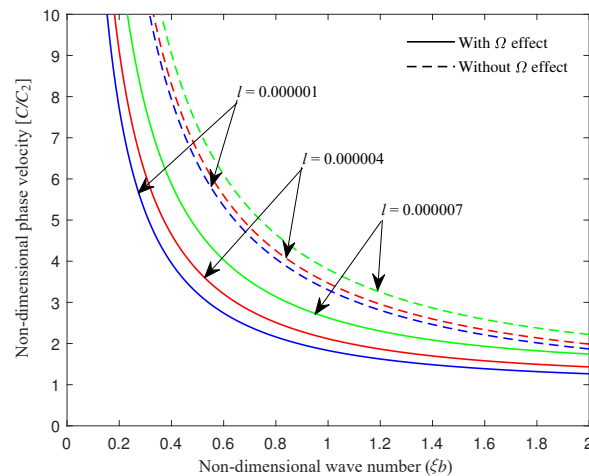
FIG. 5. Phase velocity profiles for illustrating impact of varying characteristic length ( l ) on symmetric SH-waves.
