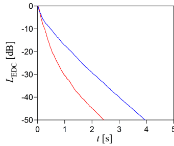
FIG. 8. Shapes of L_{\text{EDC}} at receiving point for source located in subroom A (blue line) and subroom B (red line).
