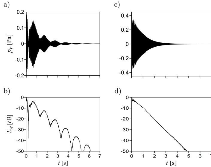
FIG. 5. Variations in of the sound pressure p_r and the pressure level L_w at receiving point for excitation frequency: a), b) 104 Hz, c), d) 257 Hz. Sound source located in subroom A.
