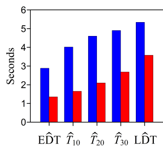
FIG. 11. Mean decay times \widehat{\text{EDT}} , \widehat{T}_{10} , \widehat{T}_{20} , \widehat{T}_{30} , \widehat{\text{LDT}} on observation plane in subroom A for source located in subrooms A (blue bars) and subroom B (red bars).
