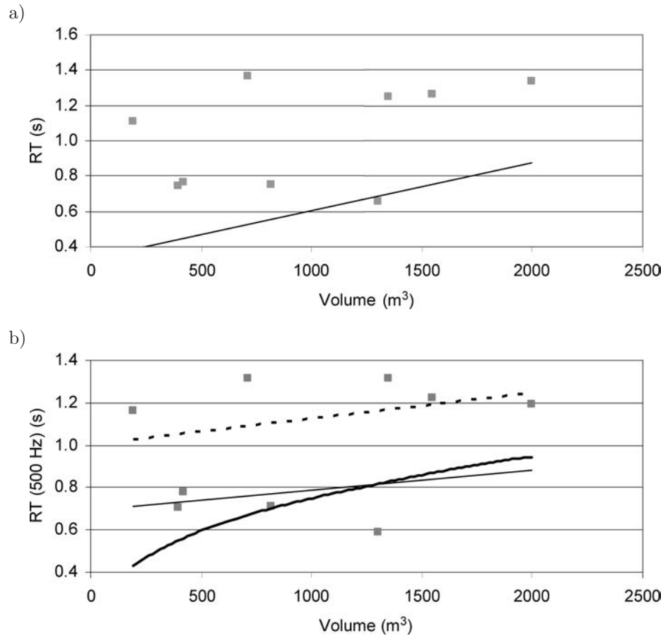
Fig. 3. Comparison between the experimentally measured and proposed optimal reverberation times: a) average experimental RT (points) and optimal value according to HODGSON (2004) (line), b) experimental 500 Hz octave value (points); optimal value proposed by KNUDSEN, HARRIS (1988) for auditoria (dashed line) and non-auditoria speech-use rooms (thin solid line); and optimal values proposed by CONTURIE (1955) for theatres and conference rooms (thick solid line).
