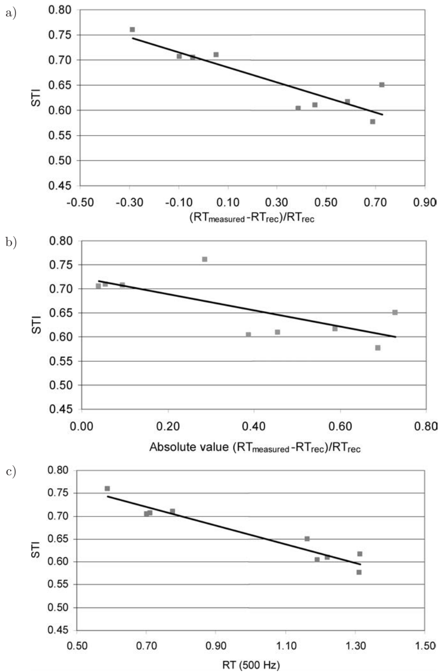
Fig. 5. a) Variation of the STI with the normalised difference among the measured reverberation time and the recommended reverberation time of Knudsen and Harris for the rooms, b) variation of the STI with the absolute value of the normalised difference mentioned in (a), c) relationship between the average STI and RT (500 Hz) for the eight rooms studied.
