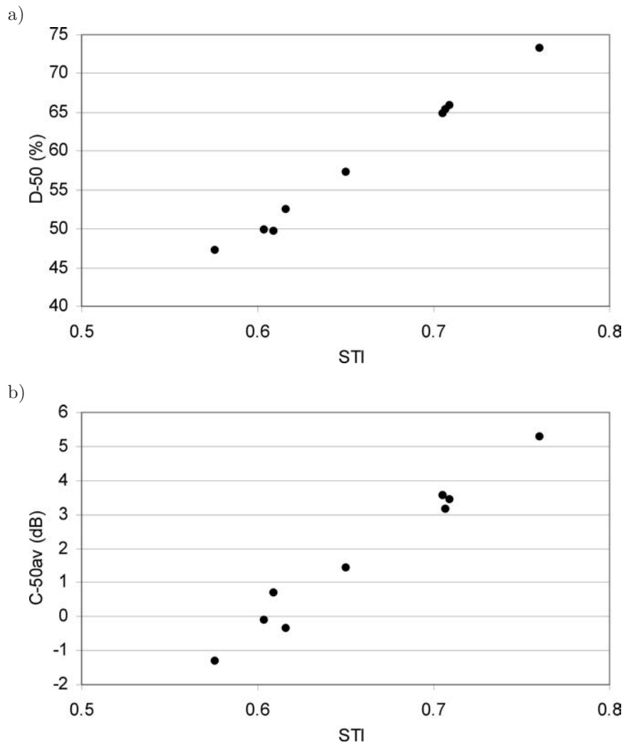
Fig. 1. Relationships between STI mean values and the other measured physical intelligibility parameters: a) Definition (D-50), b) Average Speech Clarity (C-50av).
