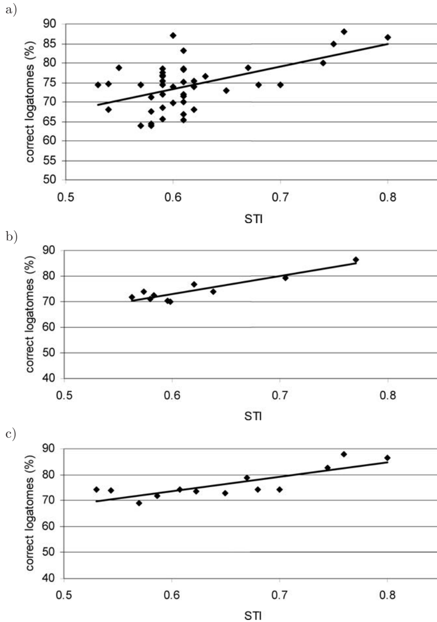
Fig. 4. a) Variation of the percentage of correct logatomes (%) as a function of the STI value for one of the rooms studied (AU1), b) the same as (a), but the results are grouped as a function of the location of the evaluation point with respect to the critical distance, c) the same as (a), but the results are grouped as a function of the STI values (in steps of 0.02).
