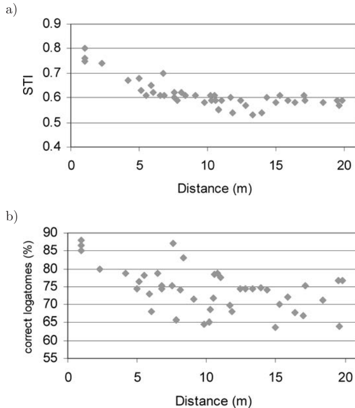
Fig. 2. Intelligibility parameters: a) variation of STI with distance for one of the rooms studied (AU1), b) variation of the percentage of correct logatomes with distance for the same room.
