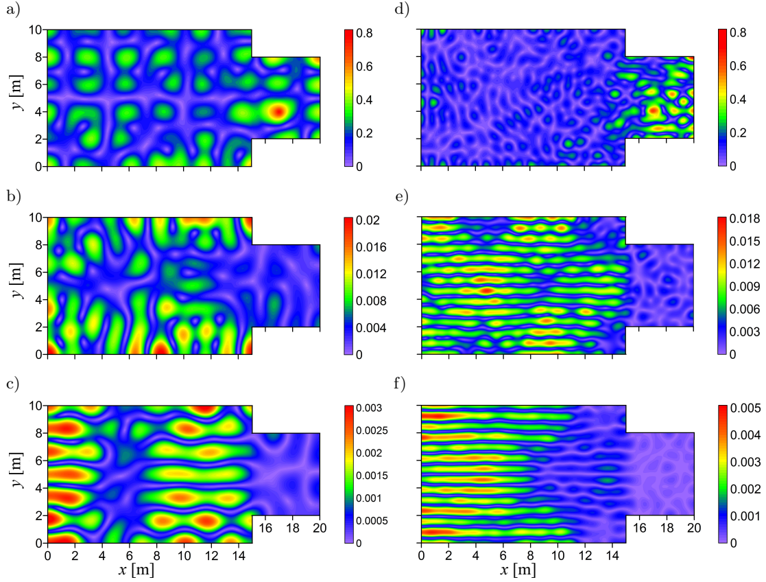
FIG. 6. Changes in the pressure amplitude P (in pascals) on observation plane for excitation frequency: a)–c) 104 Hz, d)–f) 257 Hz, and the time t : a), d) 0 s, b), e) 1 s, c), f) 2 s. Sound source located in subroom B.
